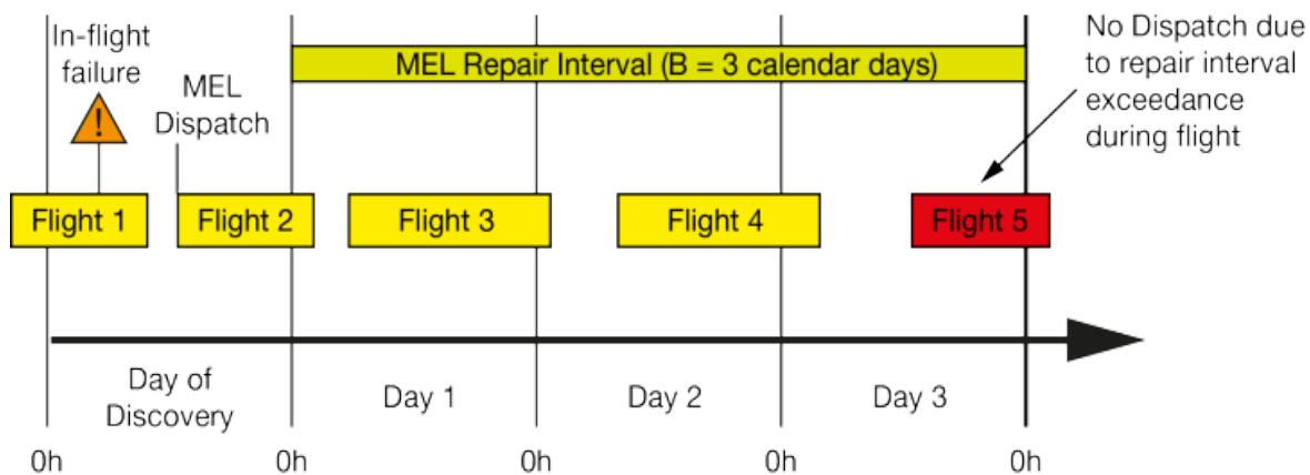
(fig.9) Principle of the repair interval
