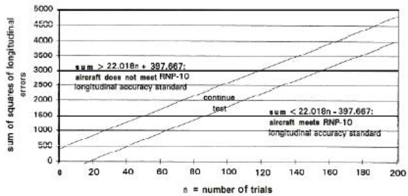
Figure 2: Acceptance, Rejection and Continuation Regions for Sequential Test of Longitudinal Accuracy
