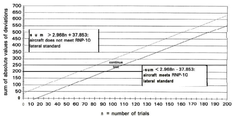
Figure 1: Acceptance, Rejection, and Continuation Regions for Sequential Test of Lateral Conformance
