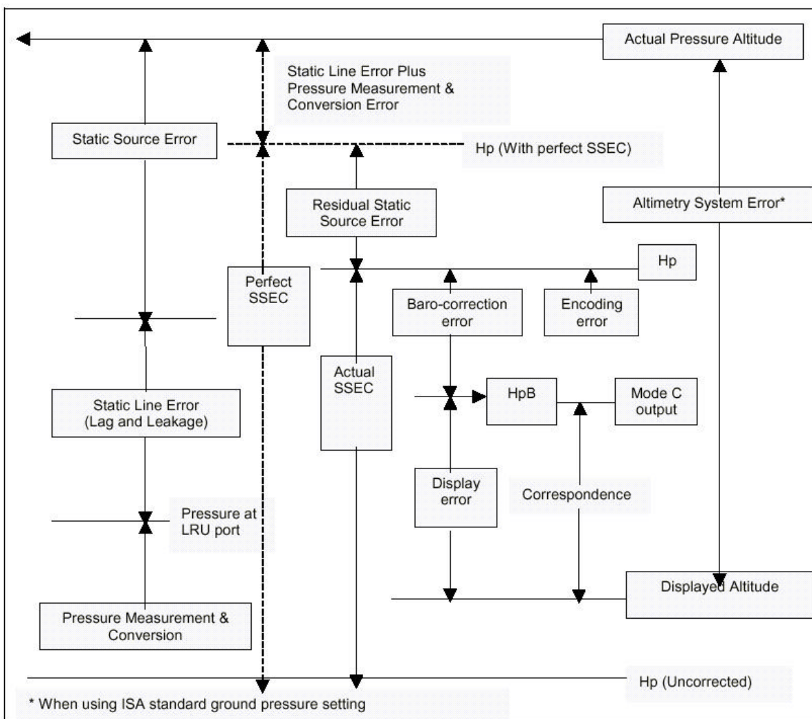
FIGURE 2-1 ALTIMETRY SYSTEM ERRORS
