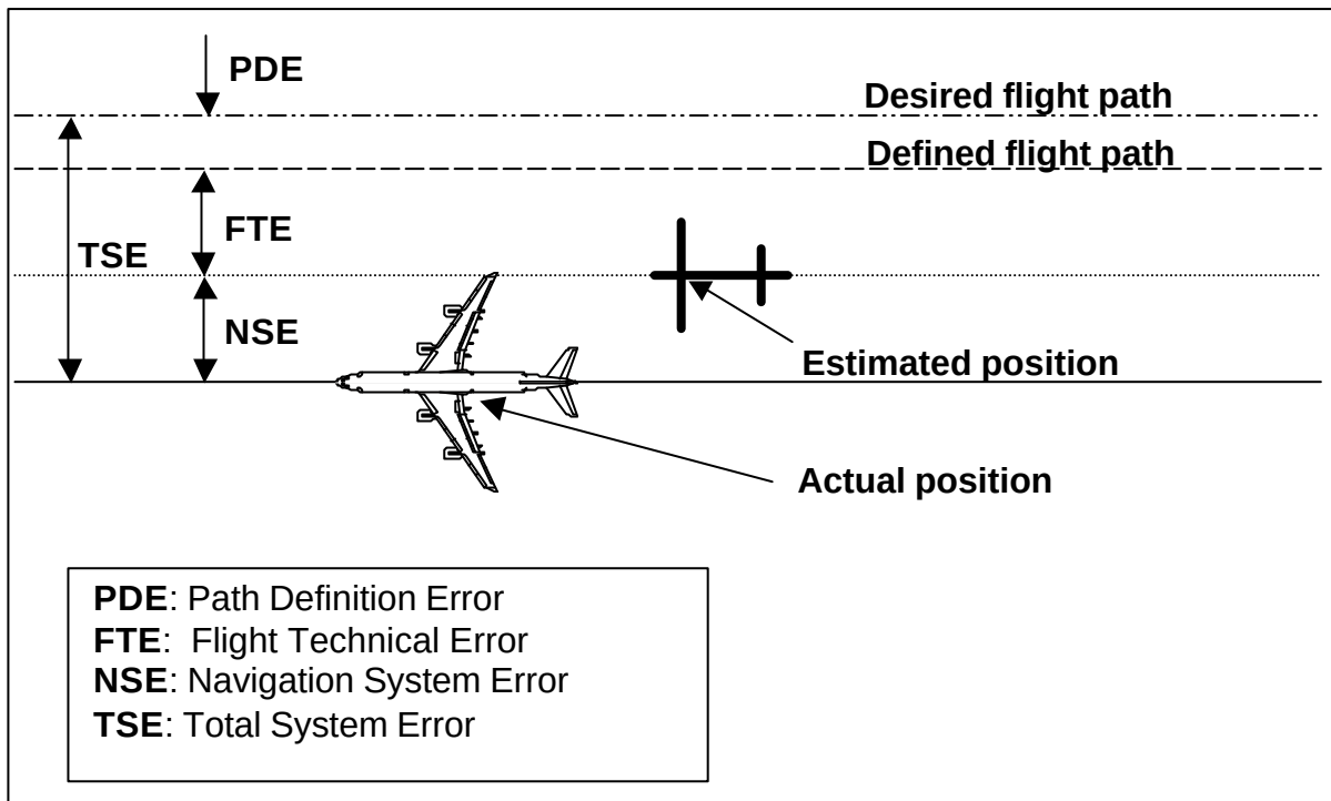
Figure 2: RNP Lateral Navigation Error Budget
