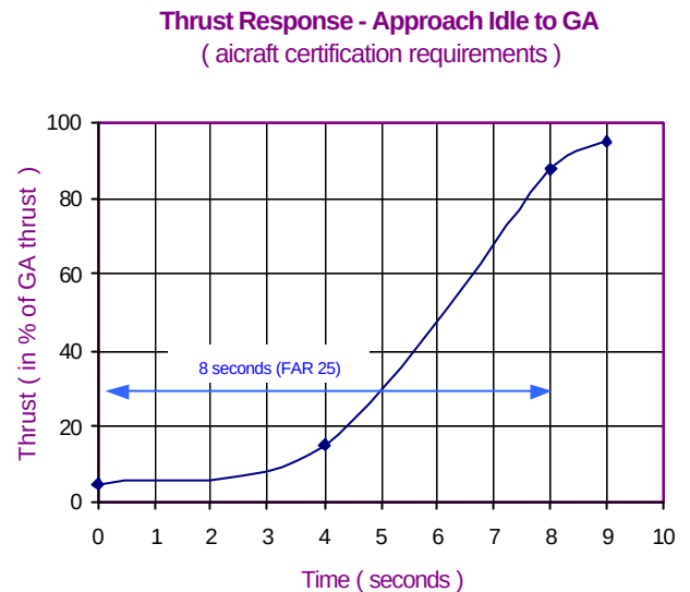
Figure 4 Certified Thrust Response -Typical
