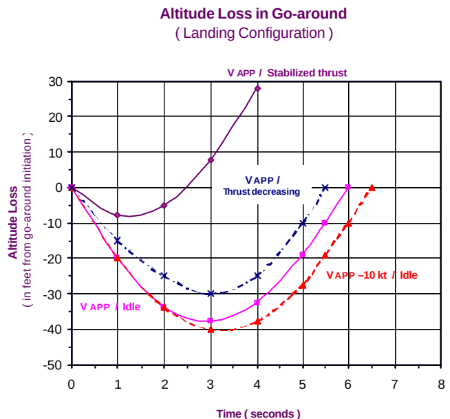
Figure 5 Effect of Initial Speed and Thrust on Altitude Loss during Go-around (Typical)
