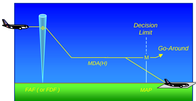
Figure 1 Step-down Final Approach
