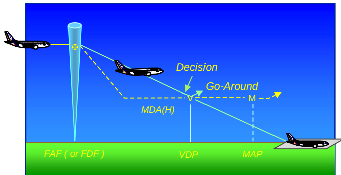
Figure 3 Constant-angle Final Approach
