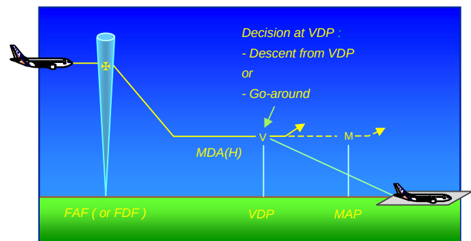
Figure 2 Visual Descent Point ( VDP ) Concept
