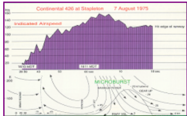
Figure 1 Wind Shear Profile - Typical
