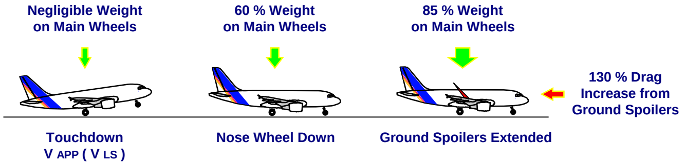
Figure 1 Maximizing Weight-on-Wheels and Aerodynamic Drag
