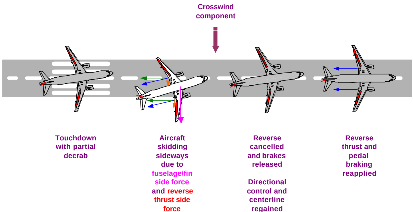
Figure 6 Directional Control during Crosswind Landing
