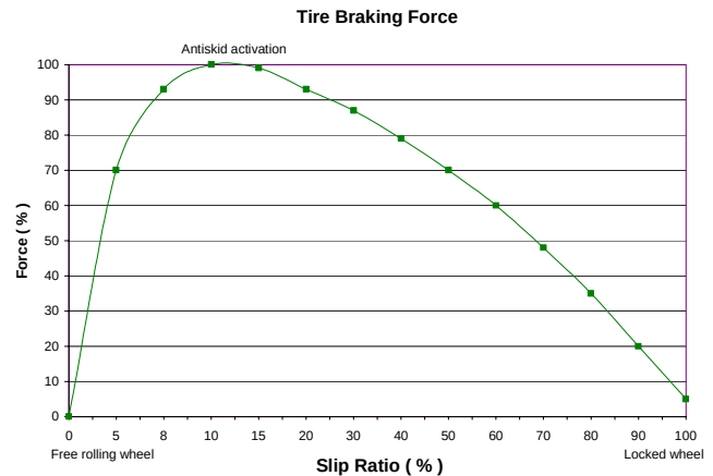
Figure 2 Tire Braking Force versus Slip Ratio
